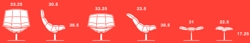
Jehs+Laub Lounge Chair and Ottoman, pedestal base
